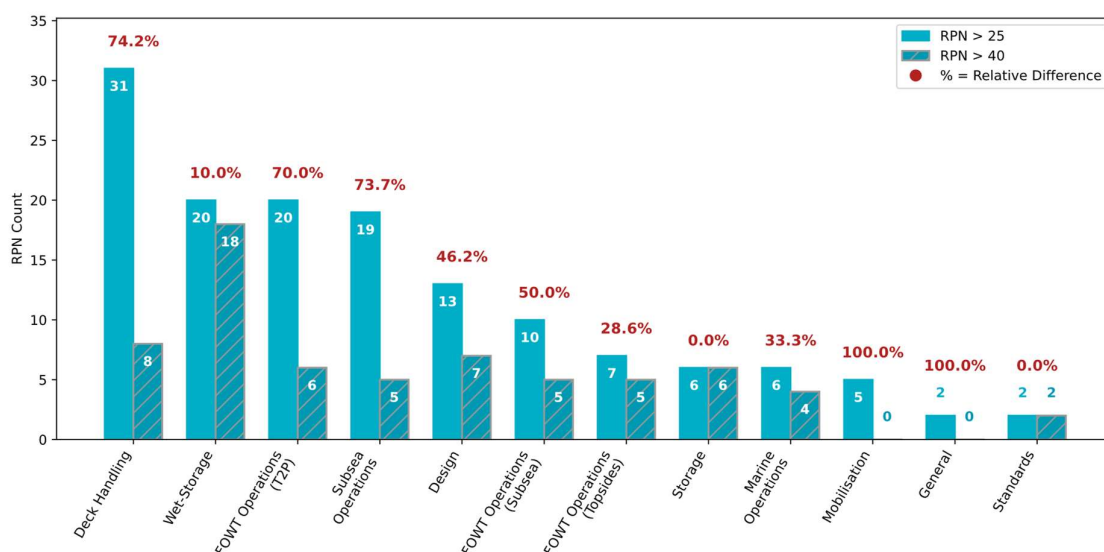
Figure 12: Comparing the counts of risks which have RPN values for each phase of the cable installation process for significant priority phases (RPN values > 25) and issues requiring urgent attention (RPN values > 40) after the risk mitigations have been applied, and the relative difference between the counts of risks occurring with these RPN values
