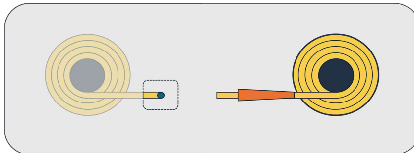
Figure 7 Sketches of a cable pull-out from a cable carousel (left) below-deck and (right) above-deck
