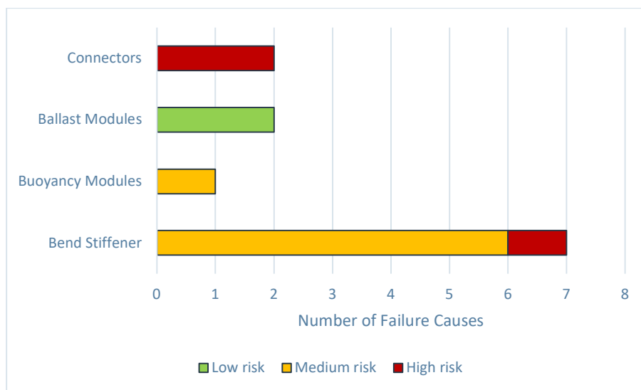
Figure 1 Failure modes per component
