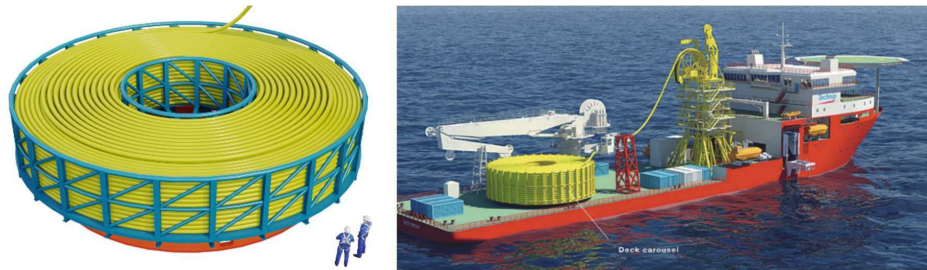
Figure 3 Back-deck cable carousel examples by (left) Maritime Developments Limited [3] and (right) Wartsila [4]
