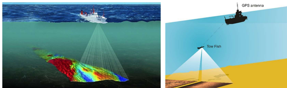
Figure 4 (left) Schematic of multi-beam echo sounder [5]; (right) Side-scan sonar [6]
