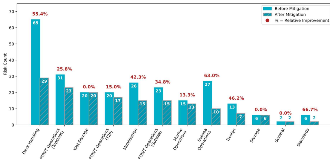
Figure 11: Counts of risk incidents for each phase of the cable installation process for high risk values (risk values > 3.5), comparing the counts of risks before mitigation to afterwards and displaying that corresponding relative improvement
